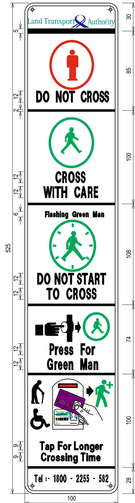
NOTE: - POSITION OF RIVETS 525mm X 100mm SCALE 1:25
