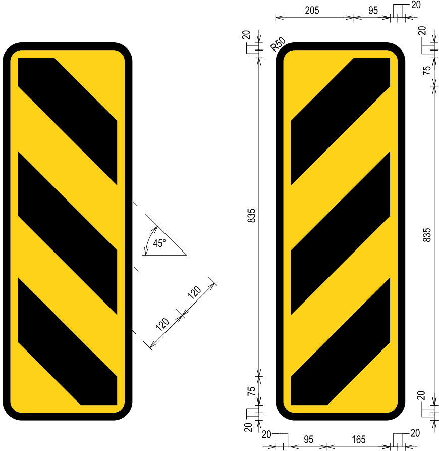
340mm X 990mm OBJECT MARKER SCALE 1:10
