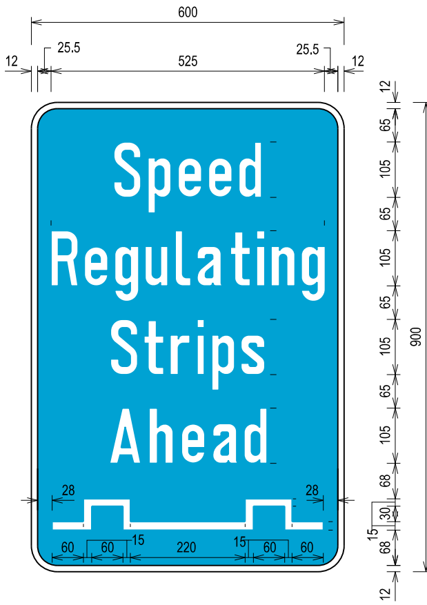
SPEED REGULATING STRIPS AHEAD THIS SIGN ADVISES MOTORISTS OF THE PRESENCE OF SPEED REGULATING STRIPS AHEAD. SPEED REGULATING STRIPS ARE USED TO SLOW DOWN VEHICLES AT LOCATIONS WHERE IT IS INADVISABLE TO TRAVEL AT A HIGH SPEED.
