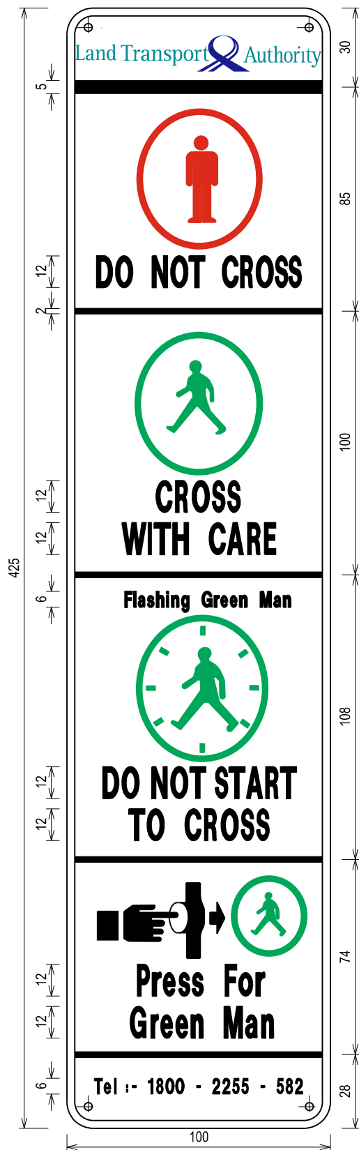
NOTE: - POSITION OF RIVETS 425mm X 100mm SCALE 1:20
