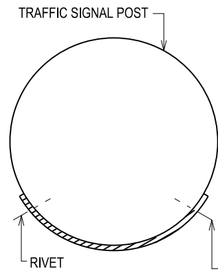
SECTION SCALE 1:1
