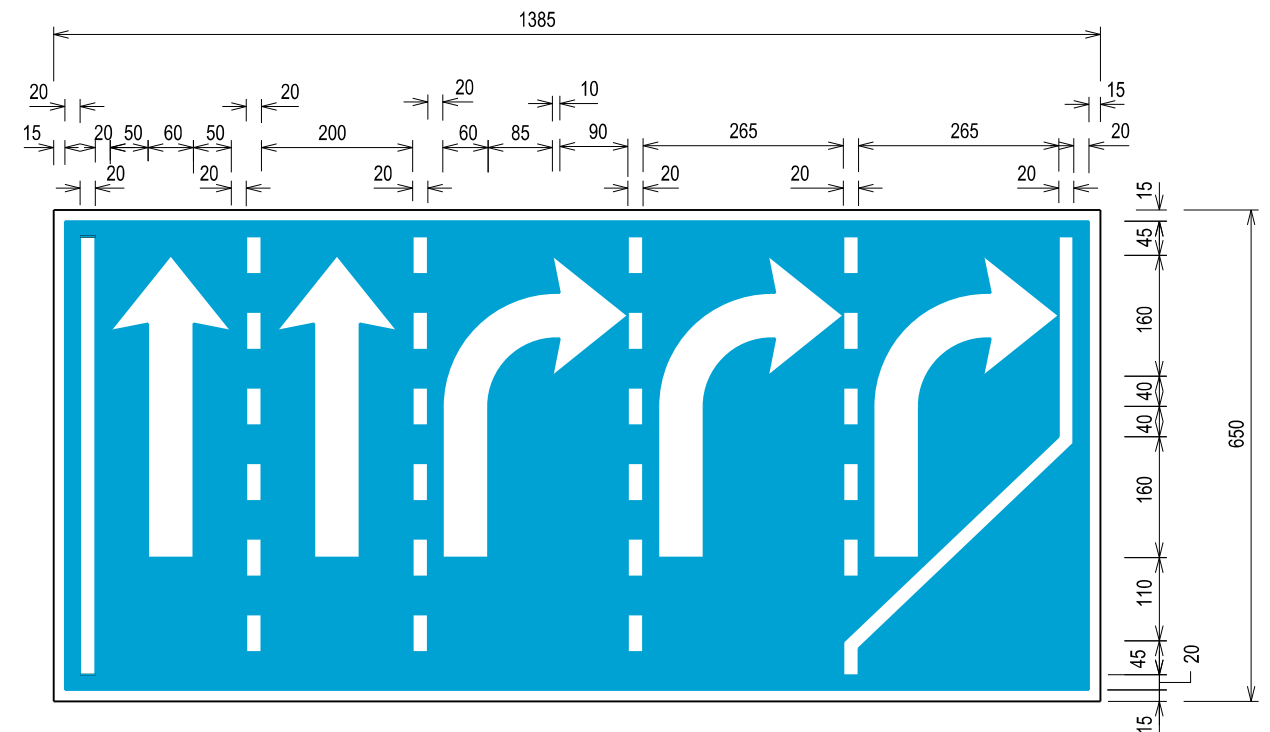
LANE INDICATION SIGN SCALE 1:10
