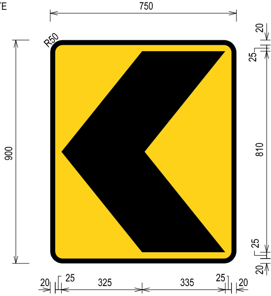
CURVE ALIGNMENT MARKER (FOR EXPRESSWAY) SCALE 1:15
