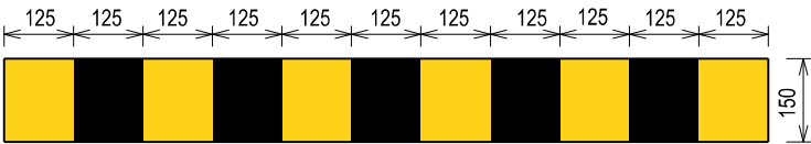
KERB STRIP MARKER SCALE 1:15
